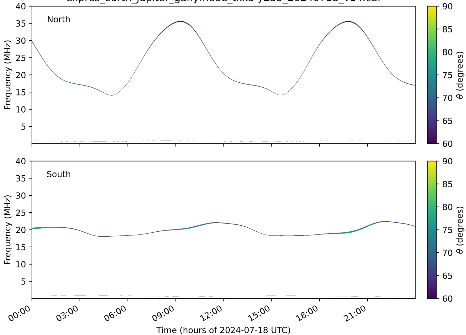
expres_earth_jupiter_ganymede_txka-y235_20240718_v14.cdf
