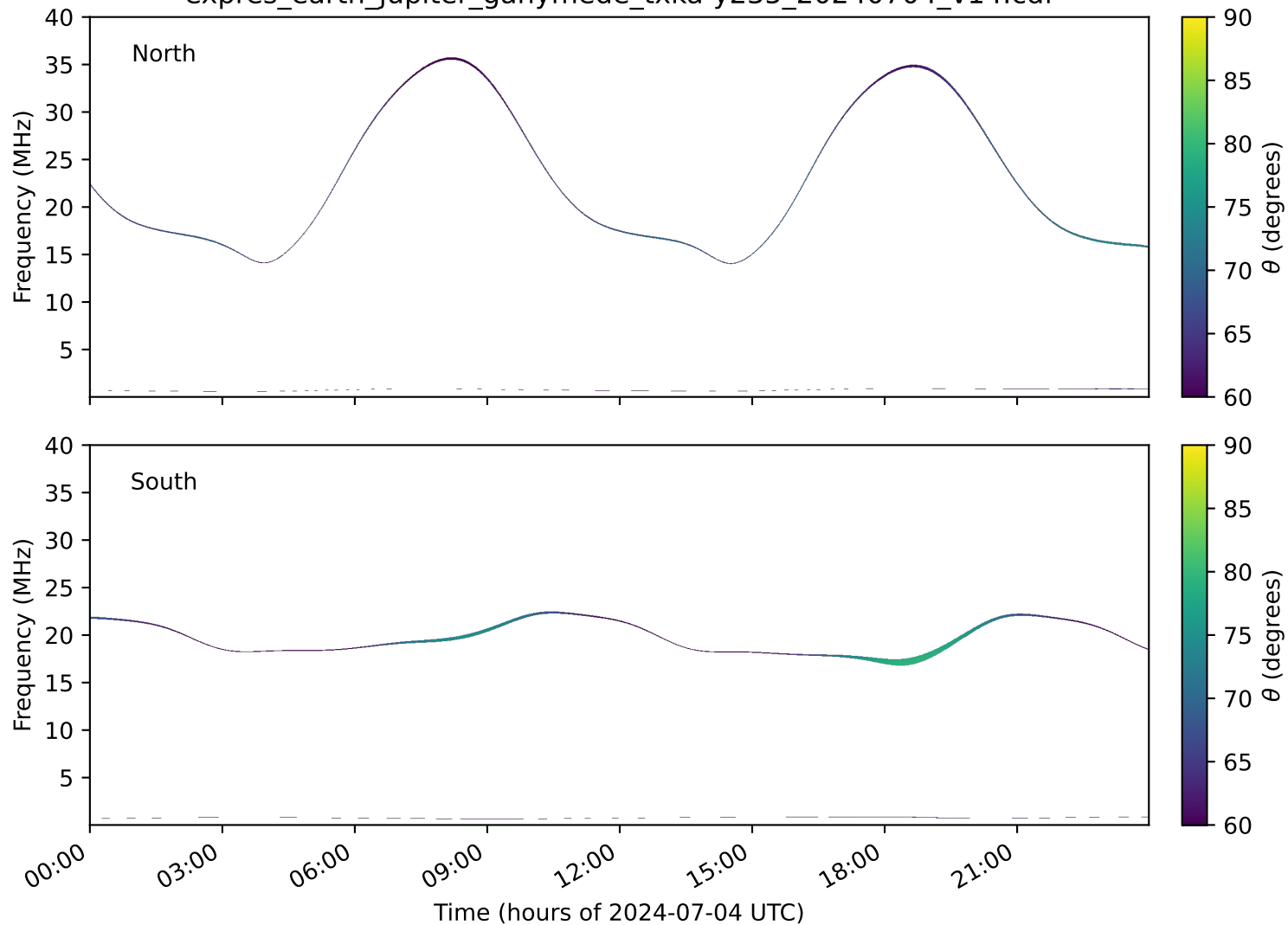
expres_earth_jupiter_ganymede_txka-y235_20240704_v14.cdf
