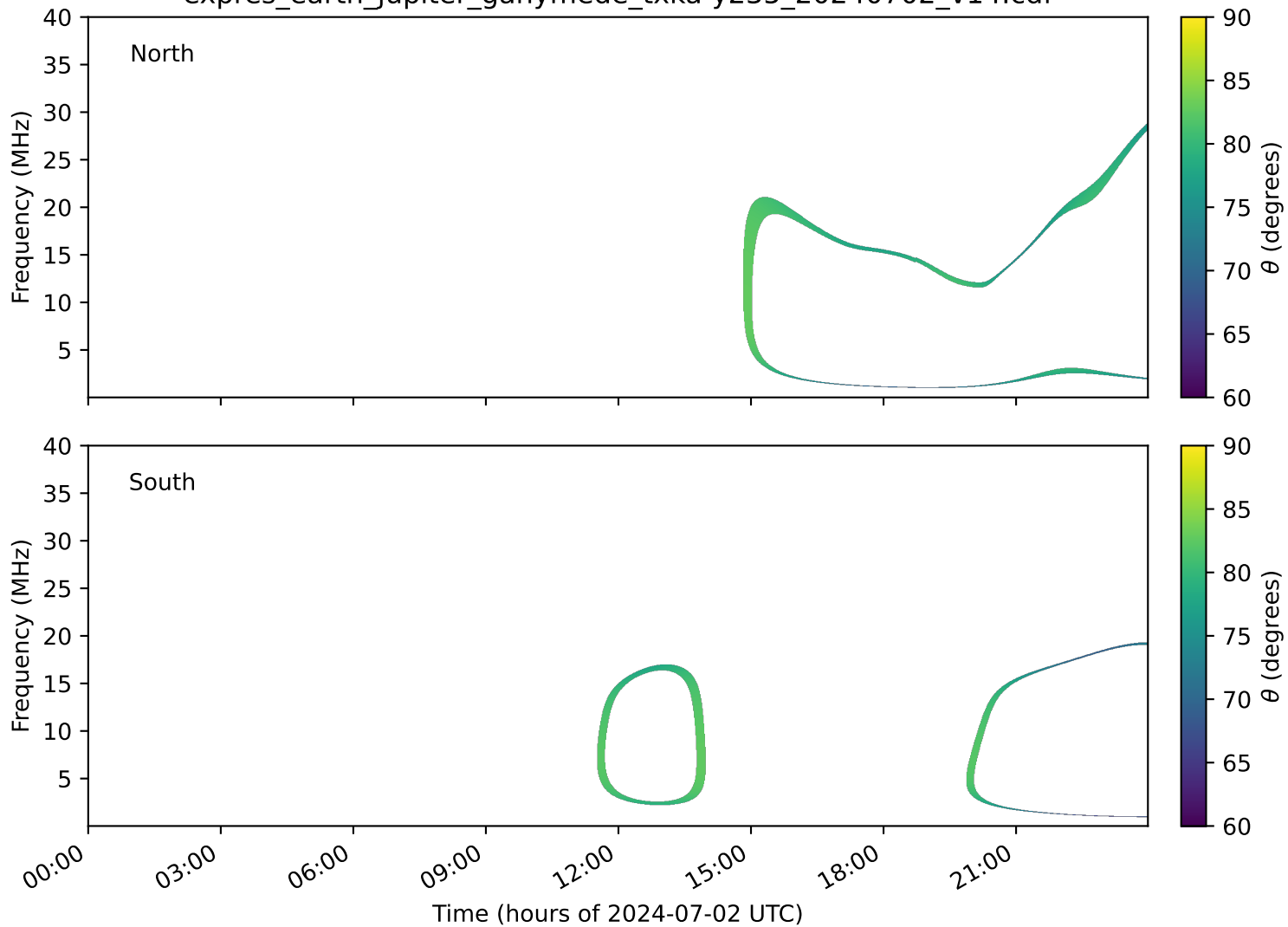
expres_earth_jupiter_ganymede_txka-y235_20240702_v14.cdf
