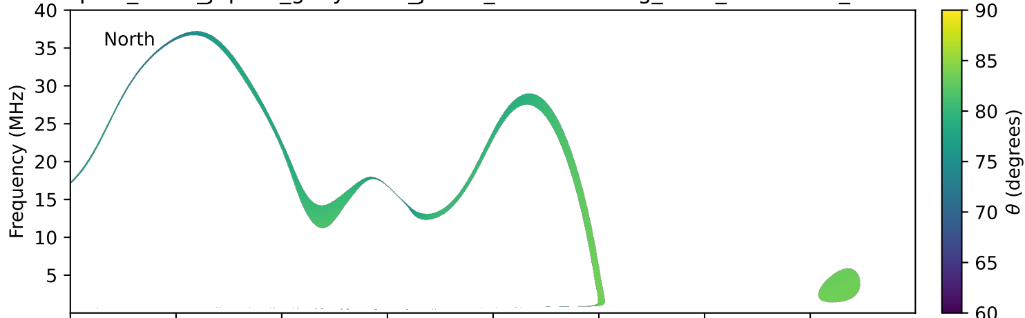
expres_earth_jupiter_ganymede_jrm33_lossc-wid1deg_3kev_20240727_v11.cdf
