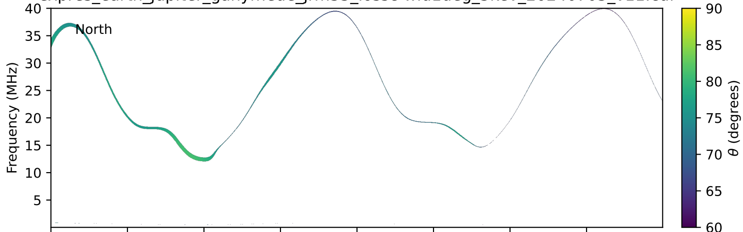
expres_earth_jupiter_ganymede_jrm33_lossc-wid1deg_3kev_20240703_v11.cdf
