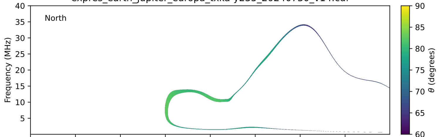
expres_earth_jupiter_europa_txka-y235_20240730_v14.cdf
