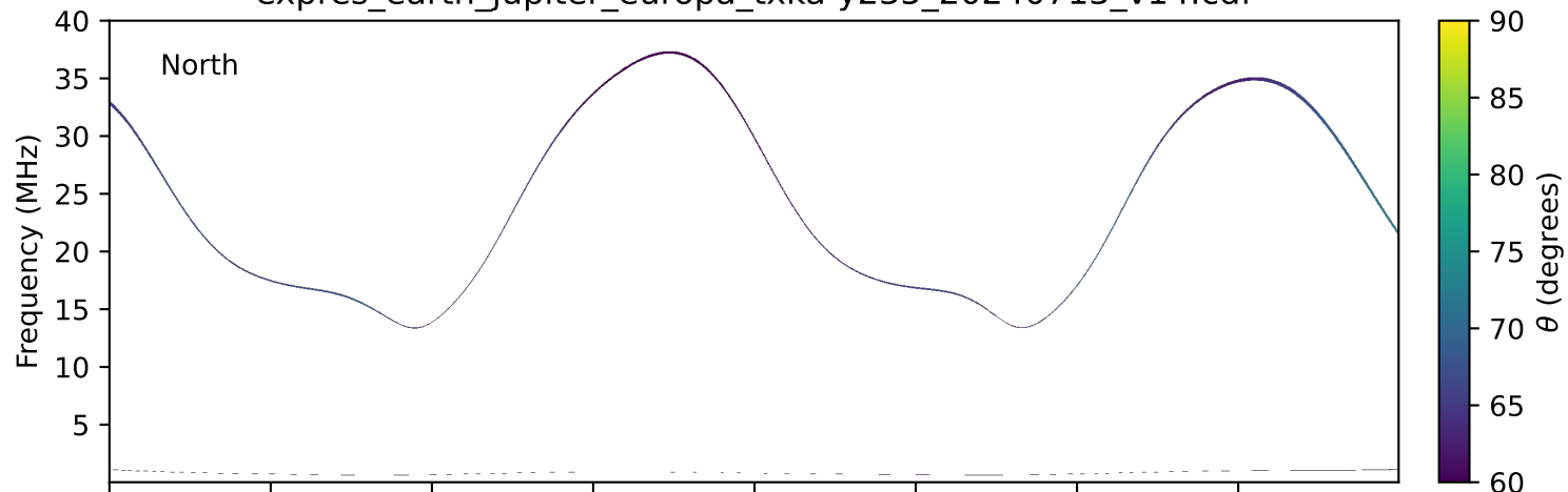
expres_earth_jupiter_europa_txka-y235_20240713_v14.cdf
