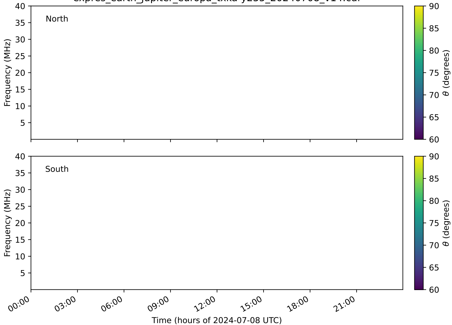
expres_earth_jupiter_europa_txka-y235_20240708_v14.cdf
