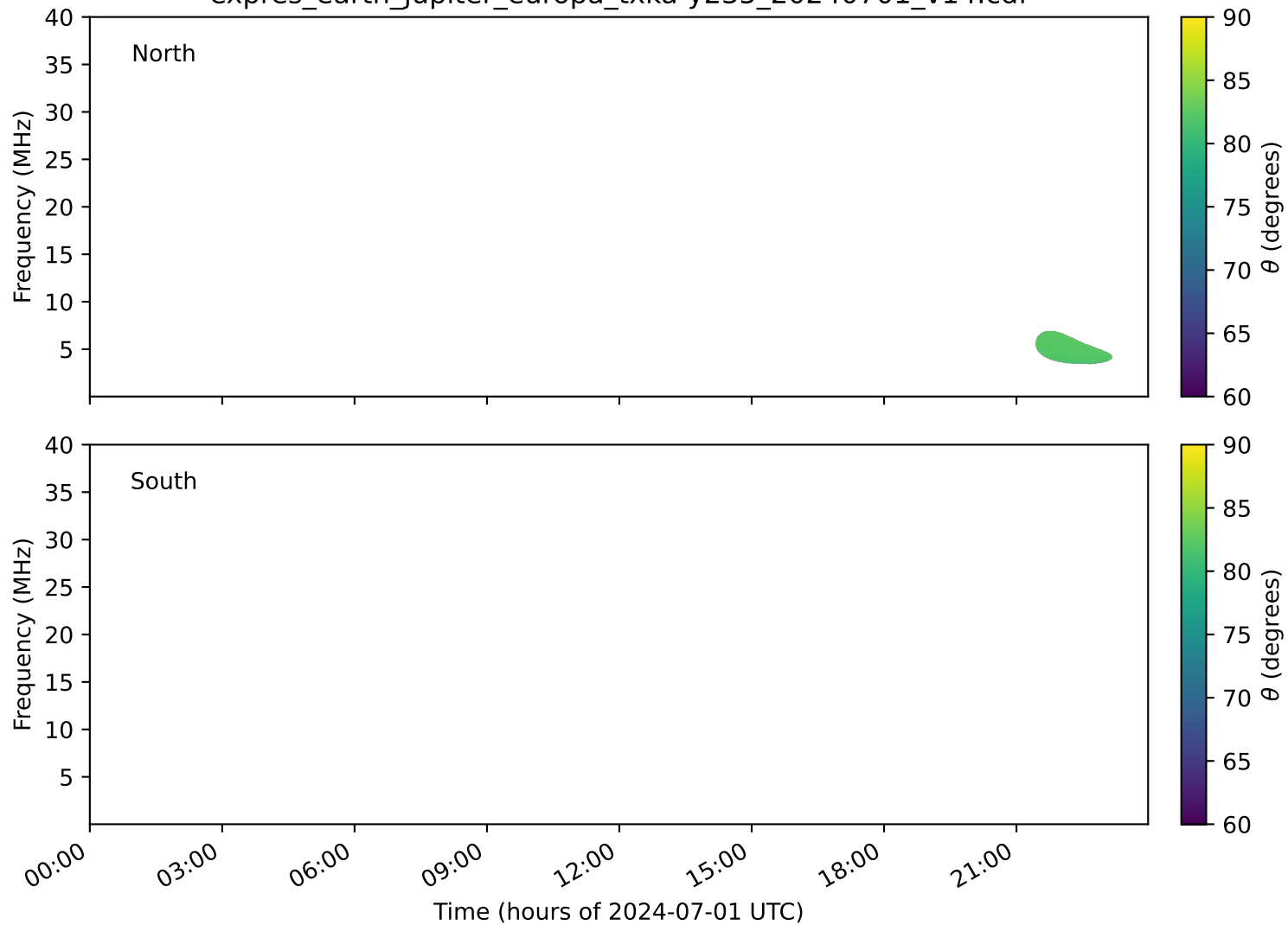
expres_earth_jupiter_europa_txka-y235_20240701_v14.cdf
