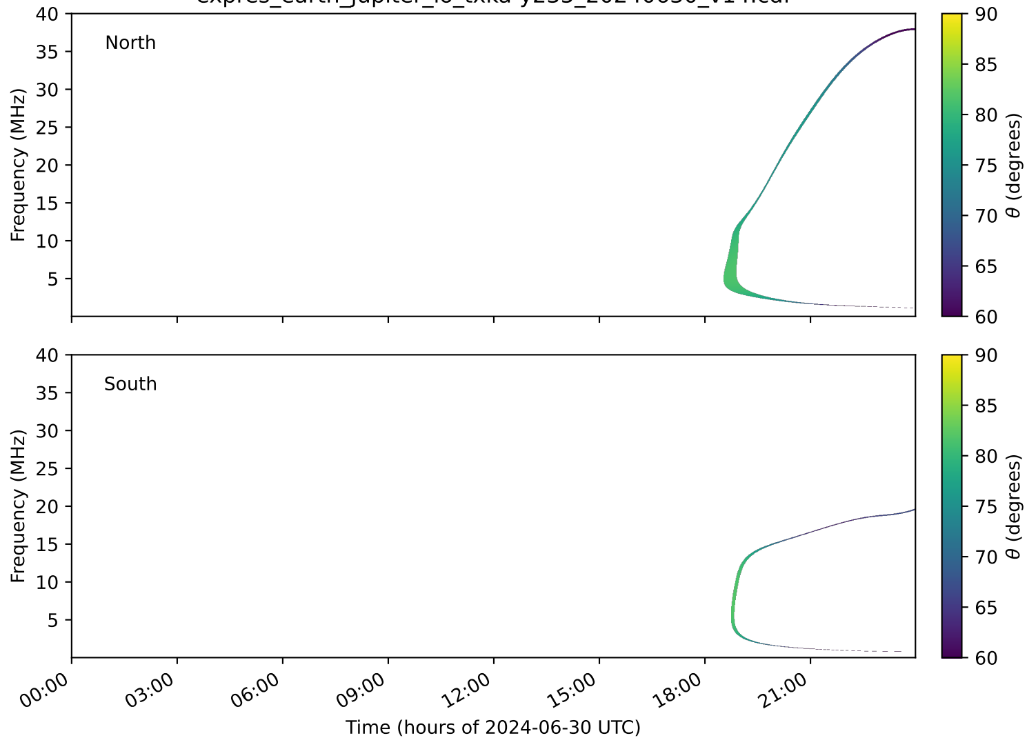
expres_earth_jupiter_io_txka-y235_20240630_v14.cdf
