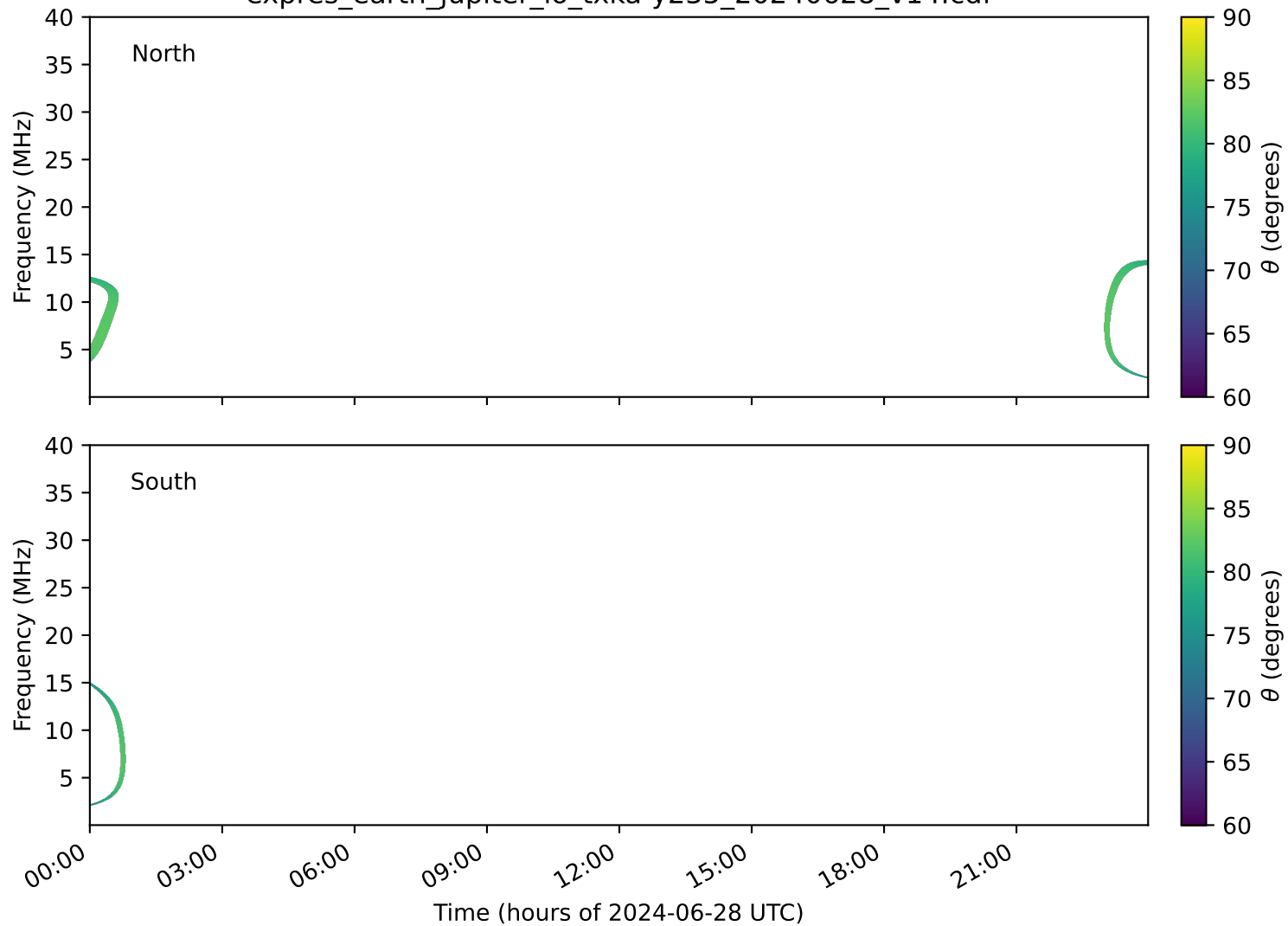
expres_earth_jupiter_io_txka-y235_20240628_v14.cdf
