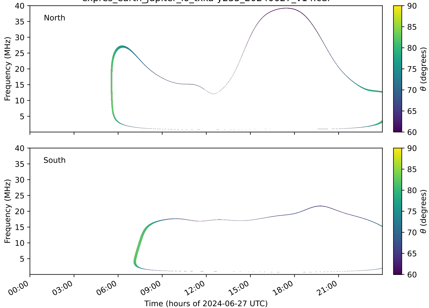
expres_earth_jupiter_io_txka-y235_20240627_v14.cdf
