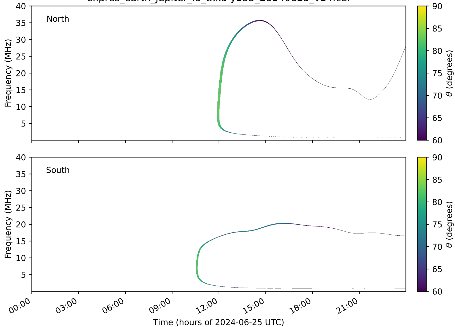
expres_earth_jupiter_io_txka-y235_20240625_v14.cdf
