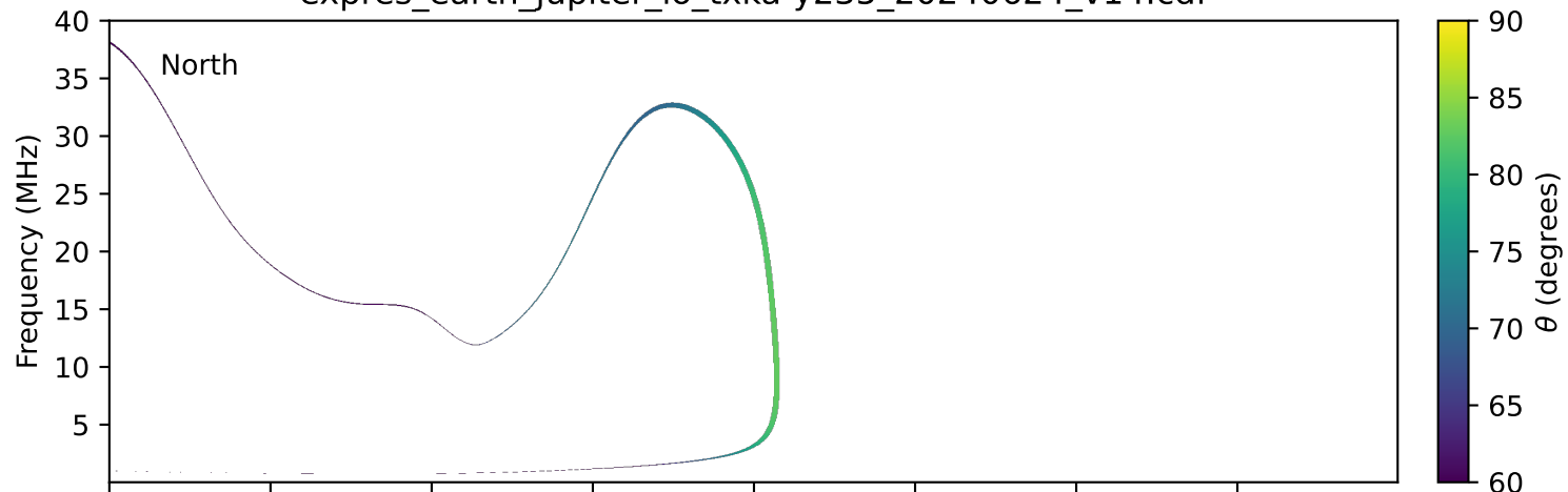
expres_earth_jupiter_io_txka-y235_20240624_v14.cdf
