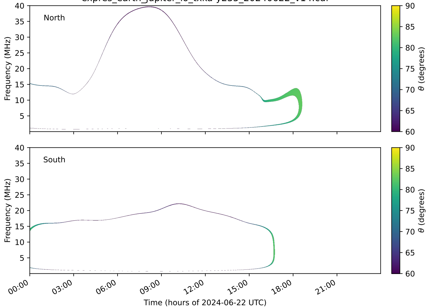
expres_earth_jupiter_io_txka-y235_20240622_v14.cdf
