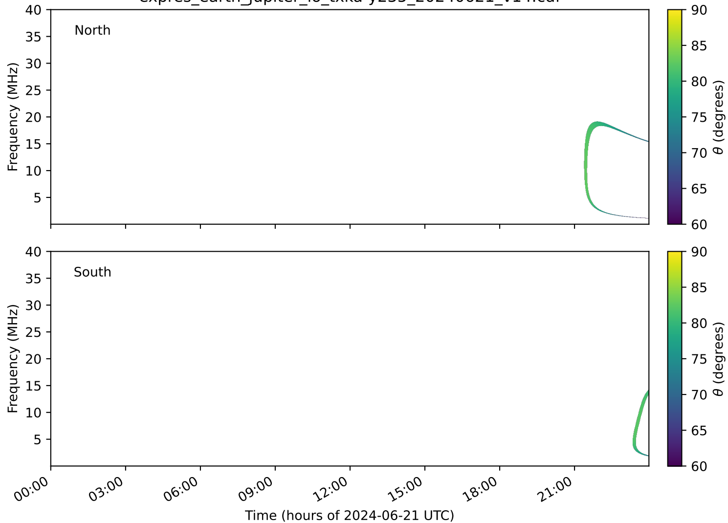
expres_earth_jupiter_io_txka-y235_20240621_v14.cdf
