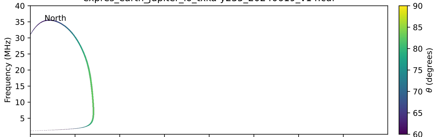
expres_earth_jupiter_io_txka-y235_20240619_v14.cdf
