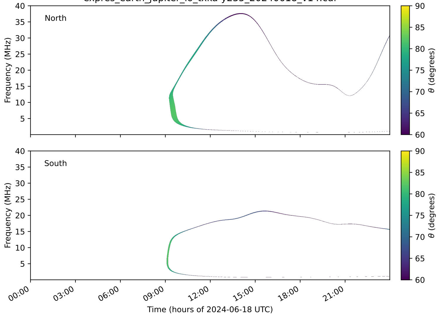
expres_earth_jupiter_io_txka-y235_20240618_v14.cdf
