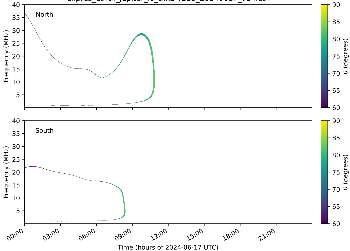
expres_earth_jupiter_io_txka-y235_20240617_v14.cdf
