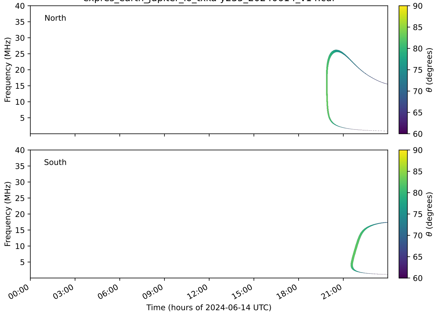
expres_earth_jupiter_io_txka-y235_20240614_v14.cdf
