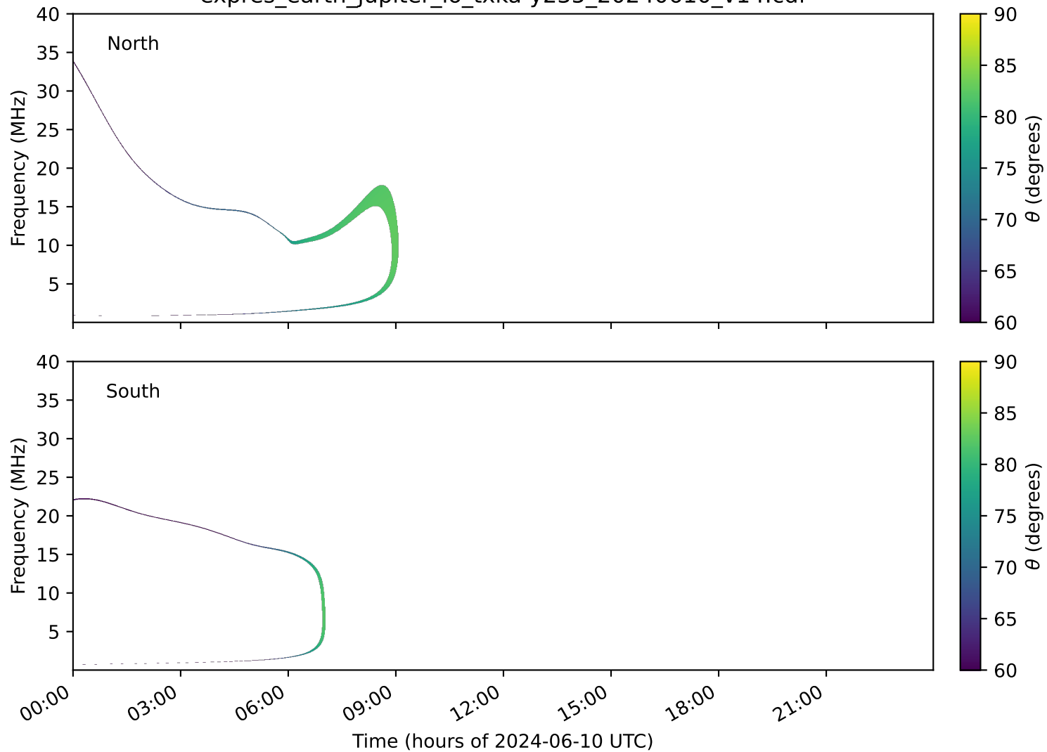
expres_earth_jupiter_io_txka-y235_20240610_v14.cdf
