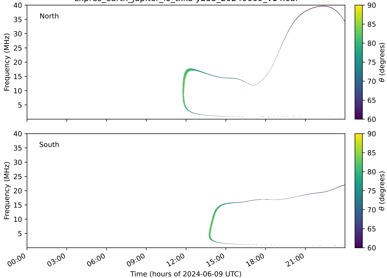
expres_earth_jupiter_io_txka-y235_20240609_v14.cdf
