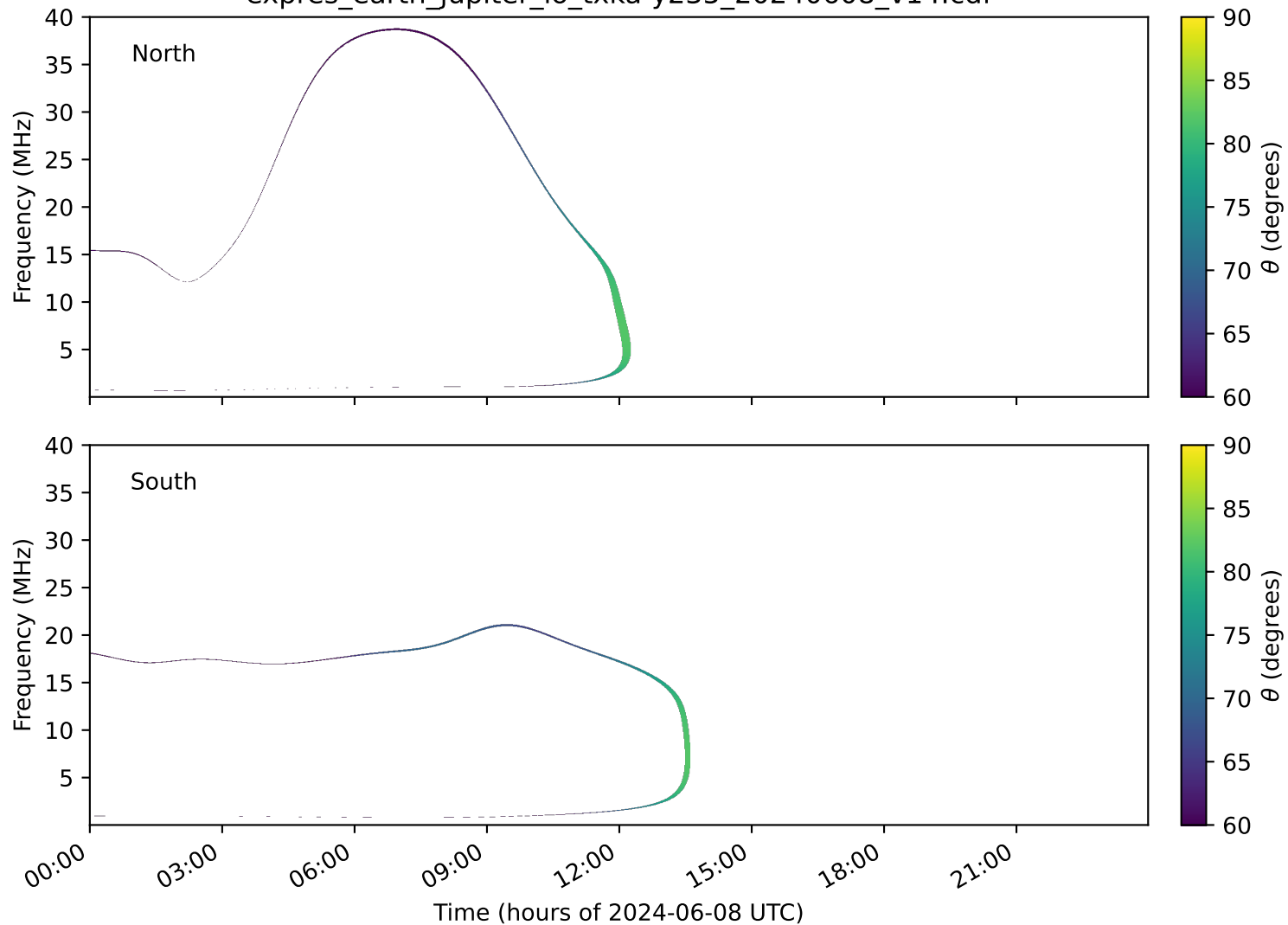
expres_earth_jupiter_io_txka-y235_20240608_v14.cdf
