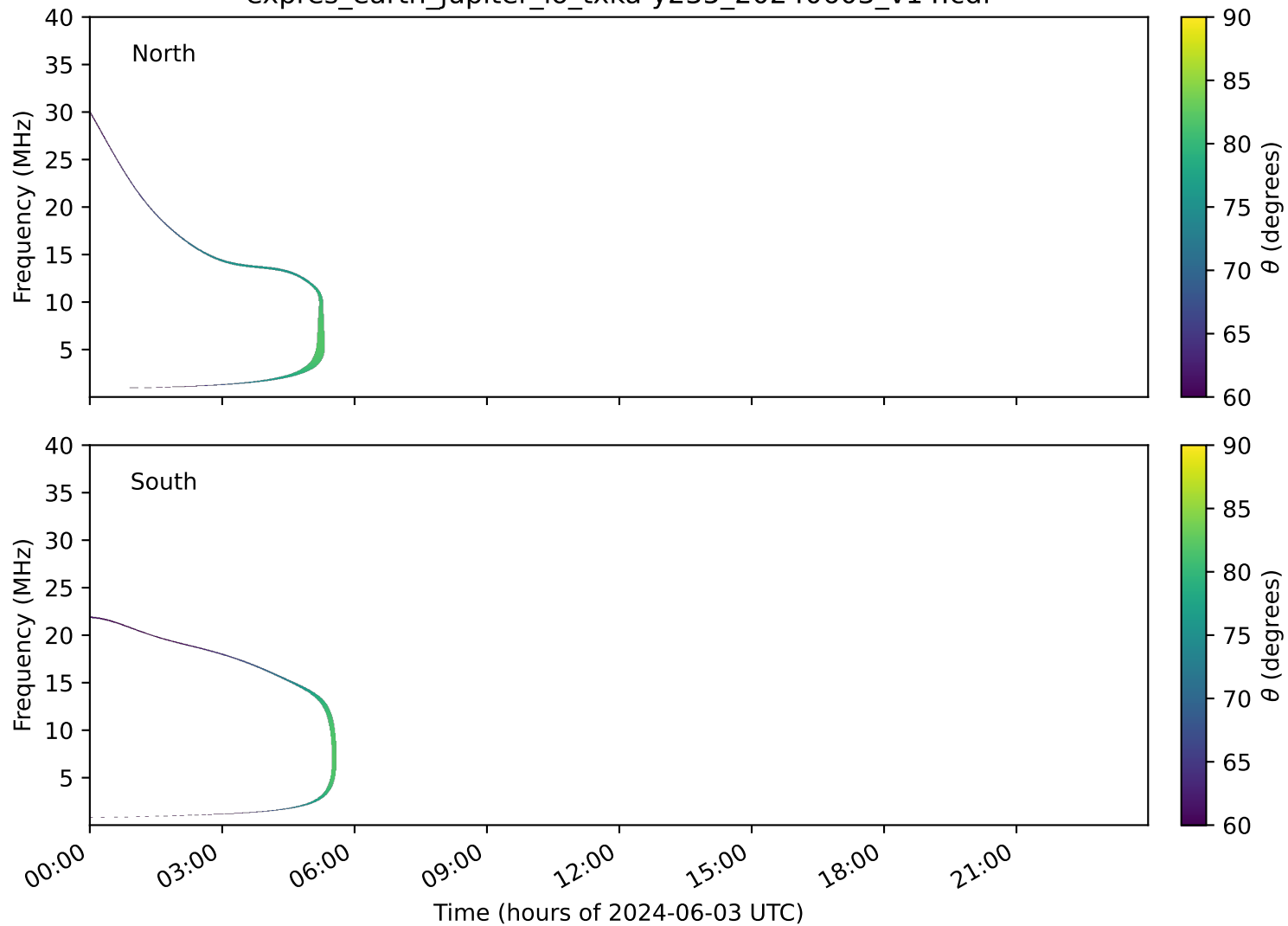
expres_earth_jupiter_io_txka-y235_20240603_v14.cdf
