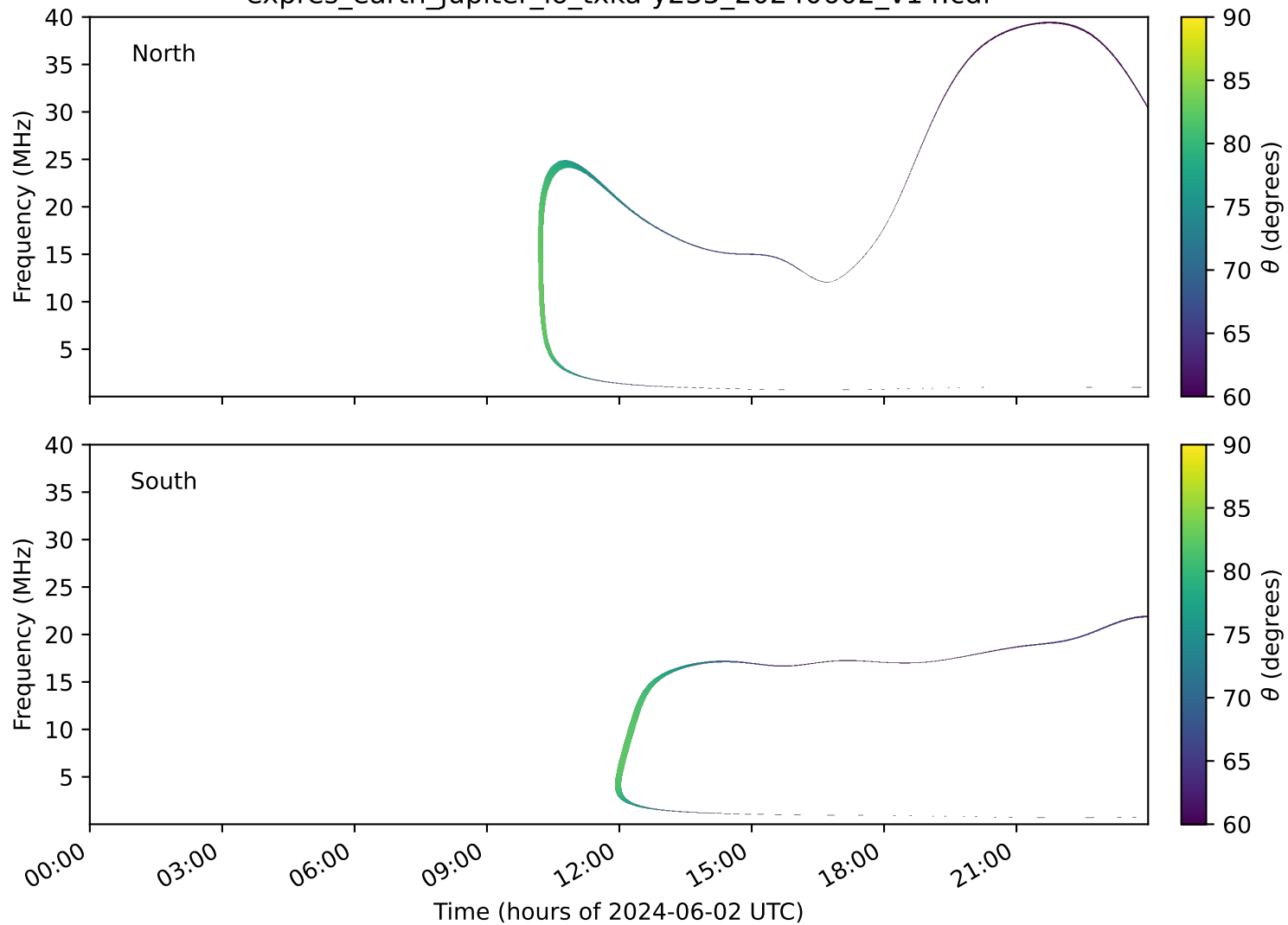
expres_earth_jupiter_io_txka-y235_20240602_v14.cdf
