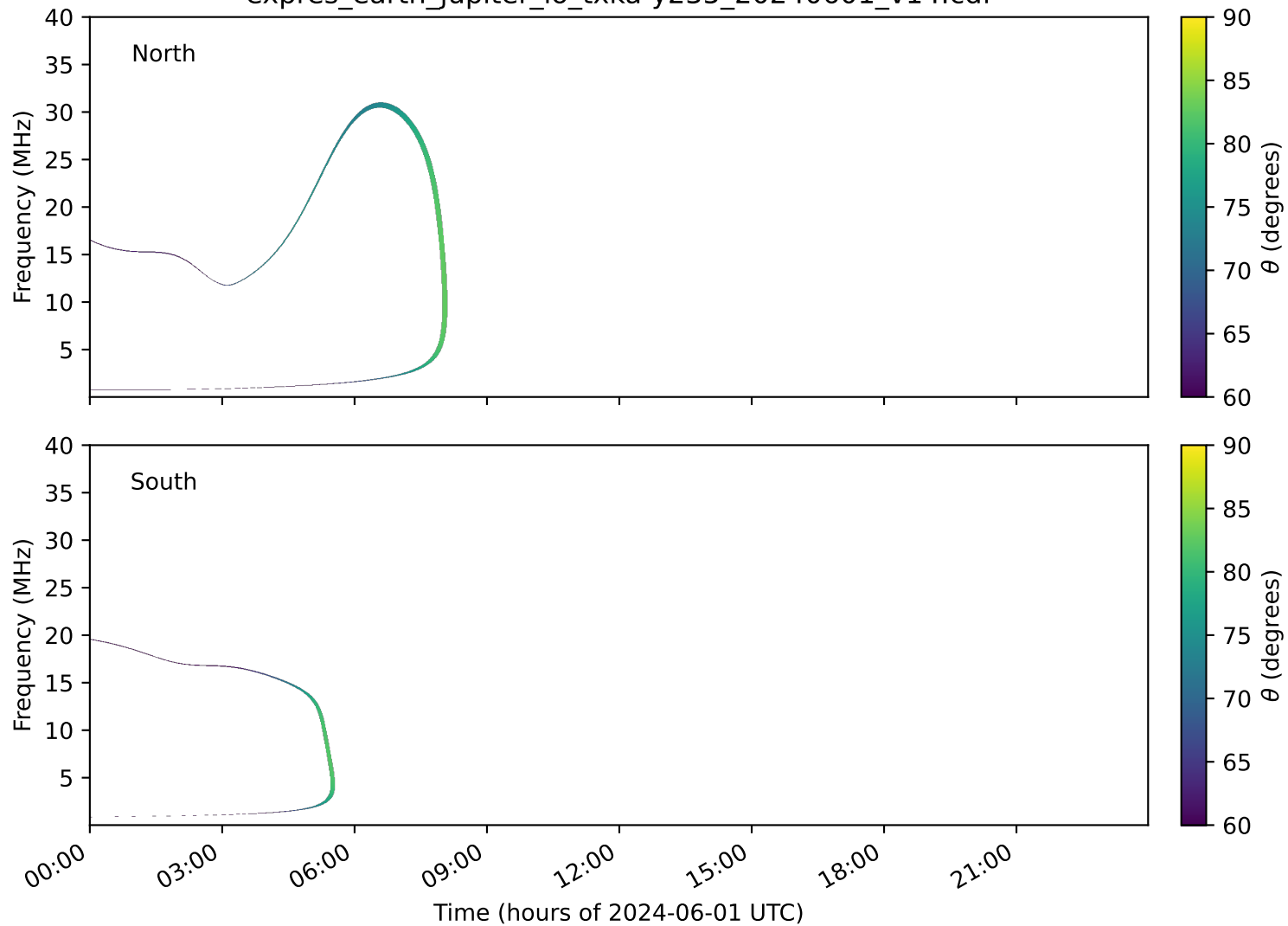
expres_earth_jupiter_io_txka-y235_20240601_v14.cdf
