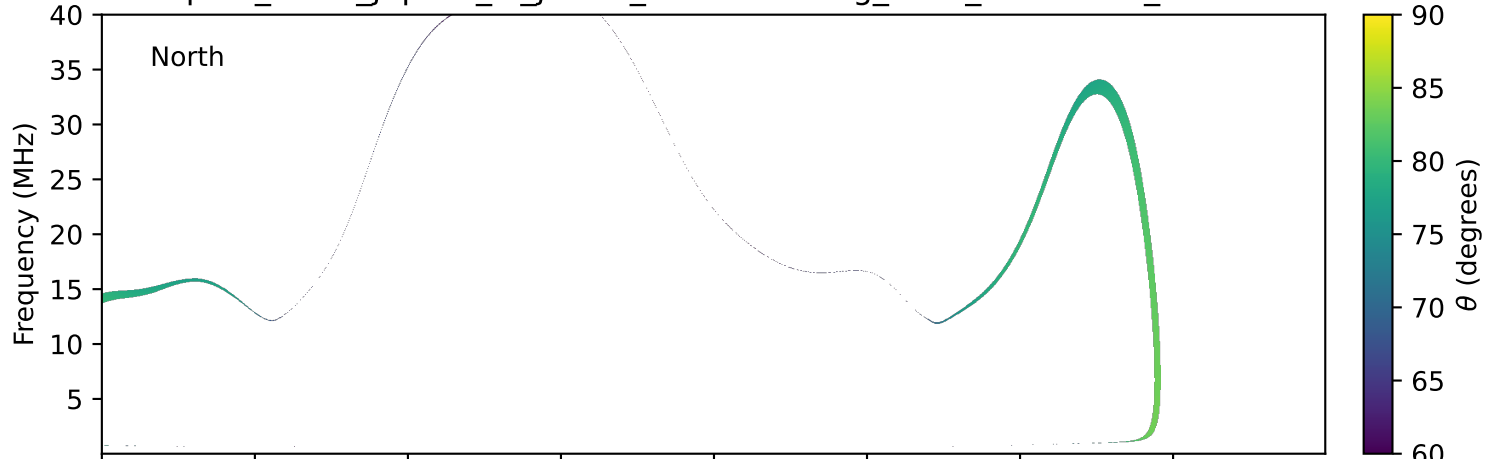
expres_earth_jupiter_io_jrm33_lossc-wid1deg_3kev_20240629_v11.cdf
