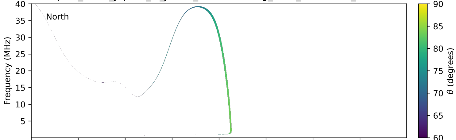
expres_earth_jupiter_io_jrm33_lossc-wid1deg_3kev_20240624_v11.cdf
