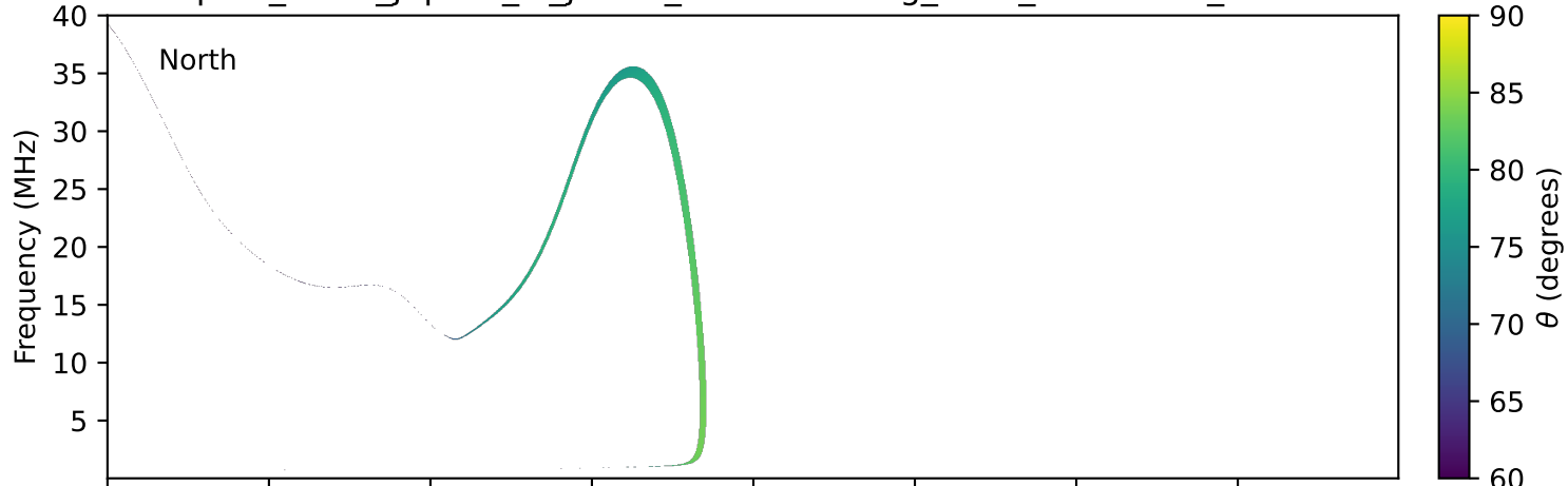
expres_earth_jupiter_io_jrm33_lossc-wid1deg_3kev_20240617_v11.cdf
