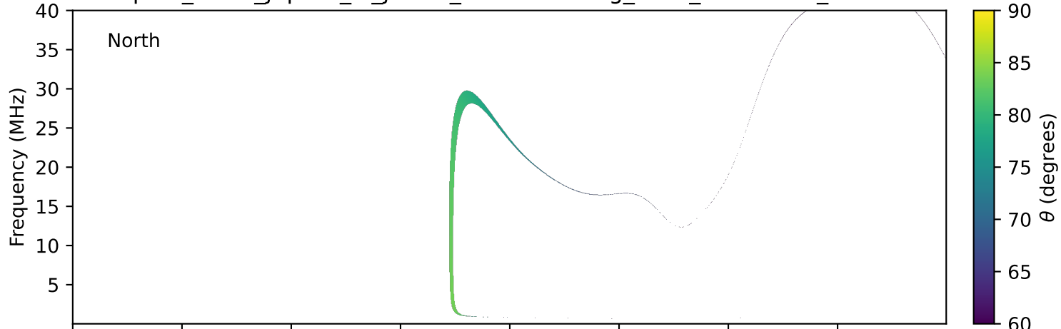
expres_earth_jupiter_io_jrm33_lossc-wid1deg_3kev_20240602_v11.cdf
