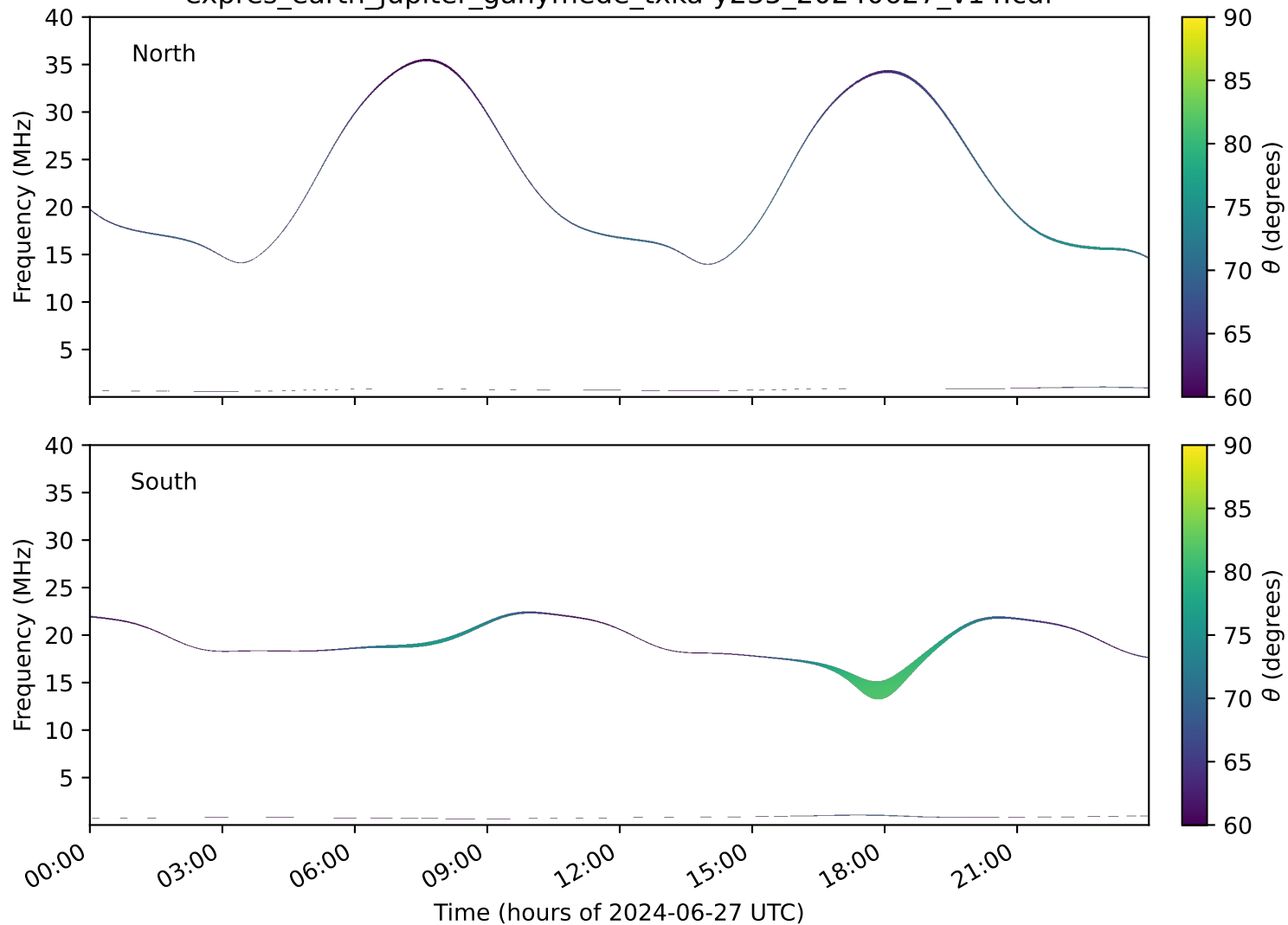
expres_earth_jupiter_ganymede_txka-y235_20240627_v14.cdf
