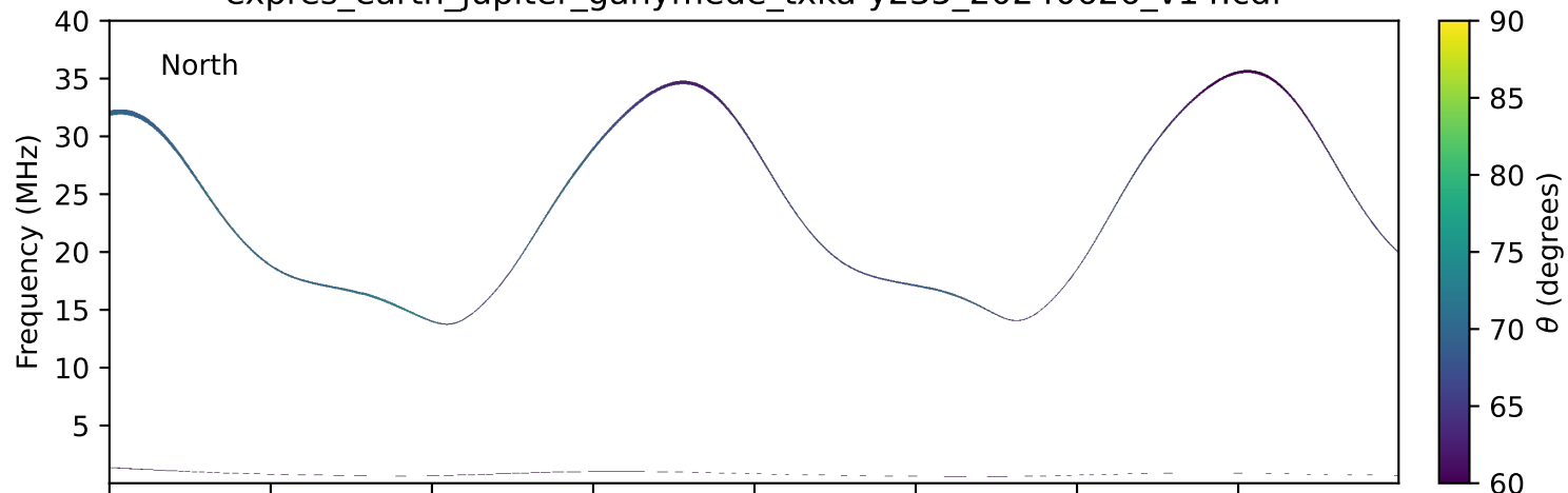
expres_earth_jupiter_ganymede_txka-y235_20240626_v14.cdf
