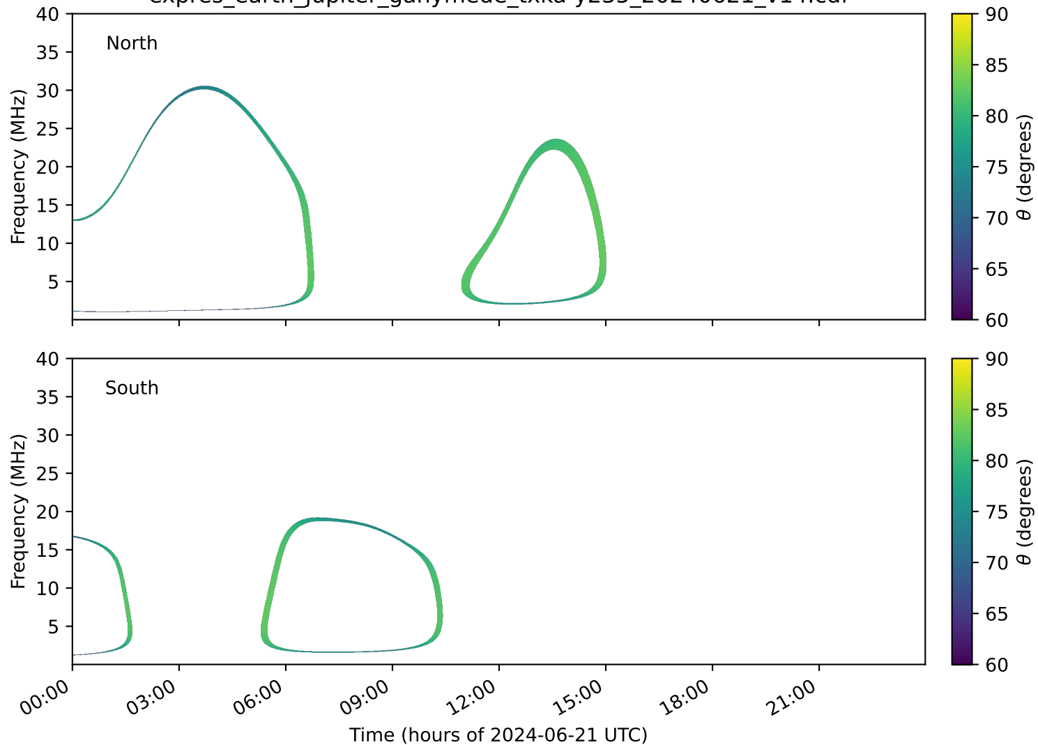
expres_earth_jupiter_ganymede_txka-y235_20240621_v14.cdf
