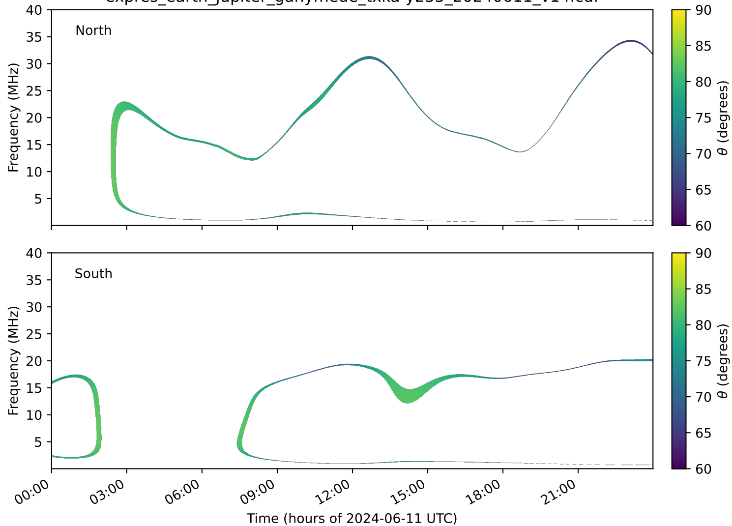
expres_earth_jupiter_ganymede_txka-y235_20240611_v14.cdf
