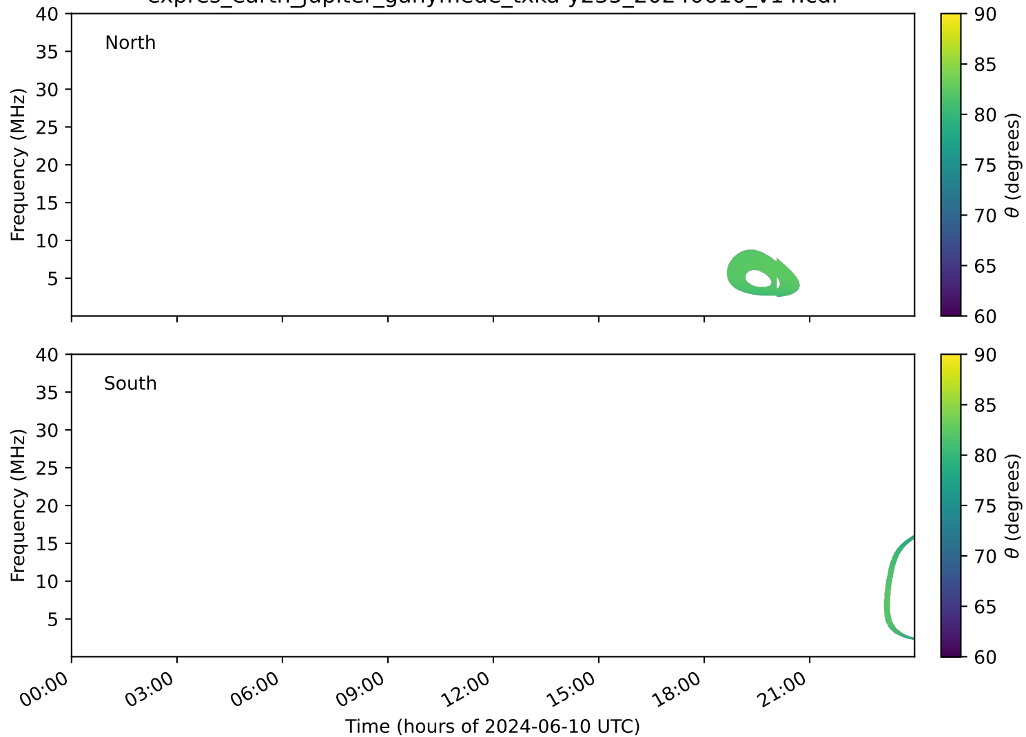
expres_earth_jupiter_ganymede_txka-y235_20240610_v14.cdf
