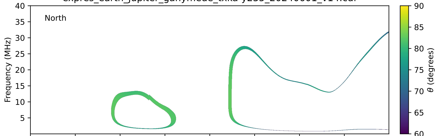
expres_earth_jupiter_ganymede_txka-y235_20240601_v14.cdf
