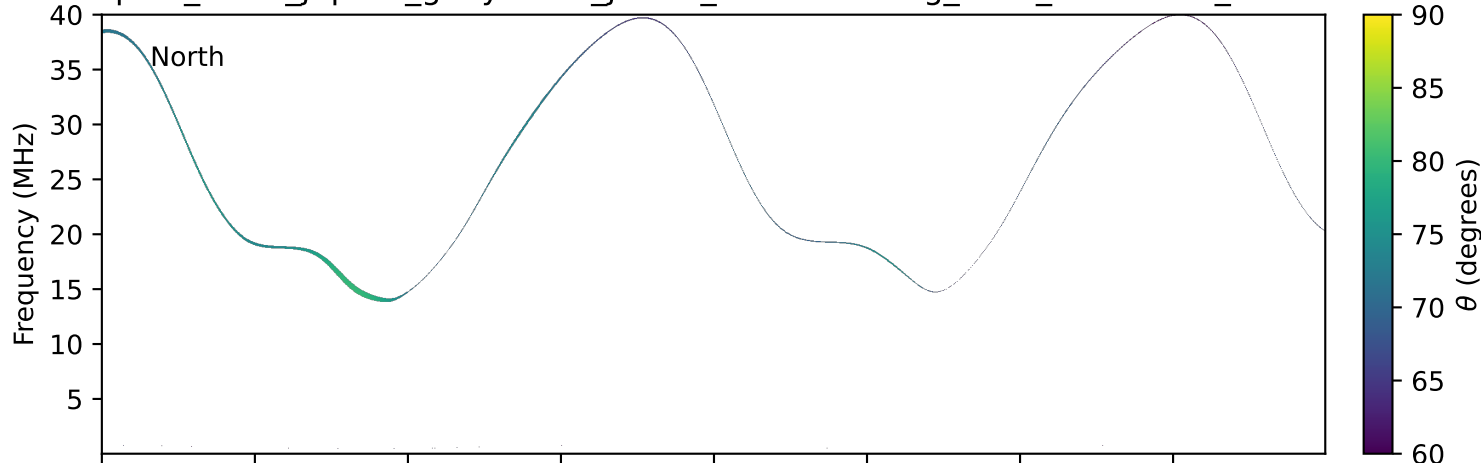
expres_earth_jupiter_ganymede_jrm33_lossc-wid1deg_3kev_20240626_v11.cdf
