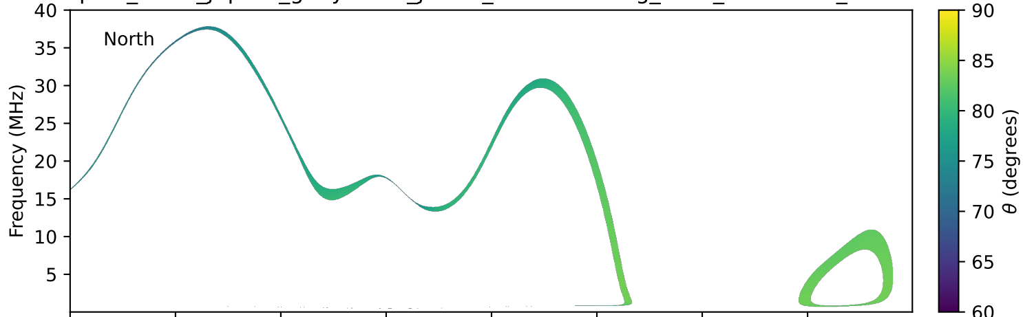
expres_earth_jupiter_ganymede_jrm33_lossc-wid1deg_3kev_20240621_v11.cdf
