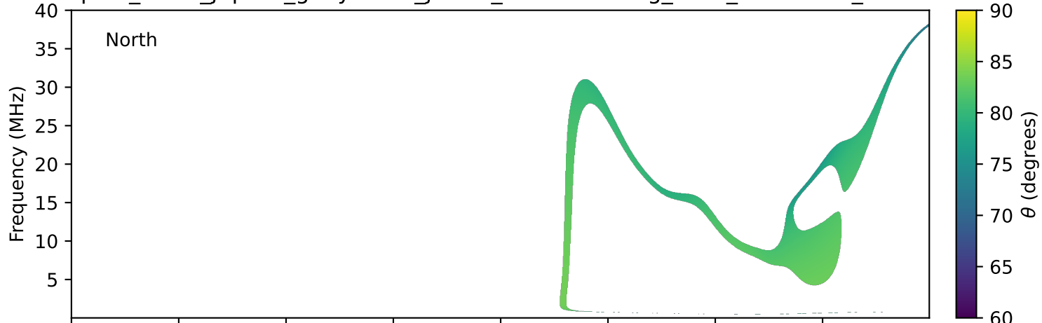
expres_earth_jupiter_ganymede_jrm33_lossc-wid1deg_3kev_20240601_v11.cdf
