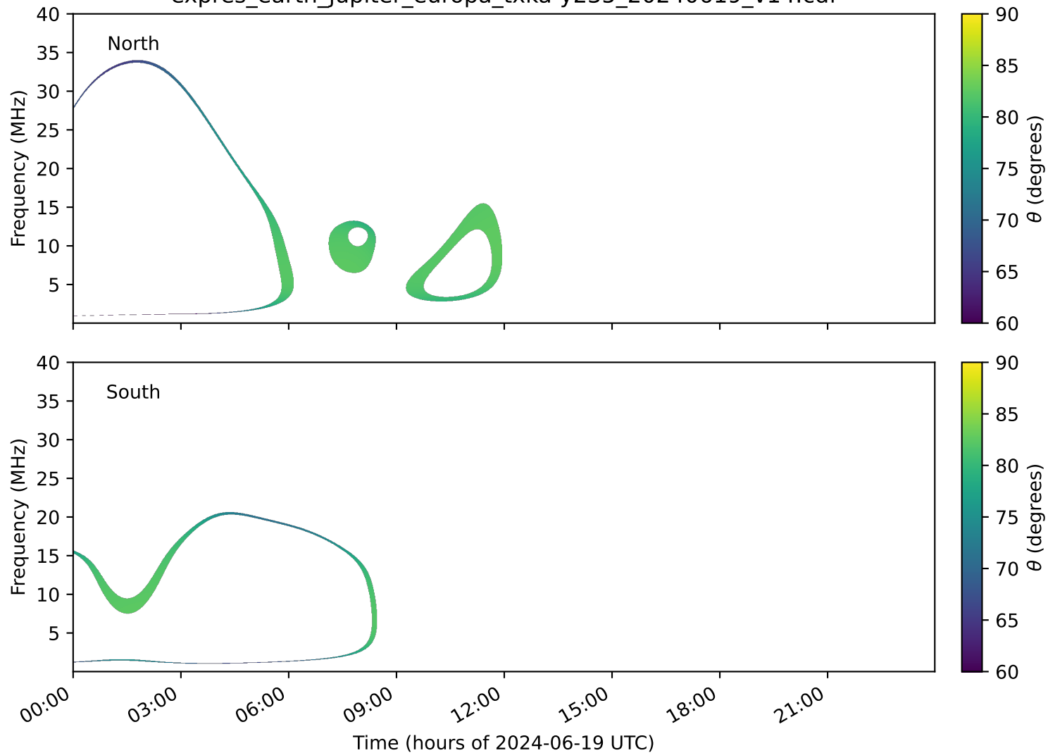
expres_earth_jupiter_europa_txka-y235_20240619_v14.cdf
