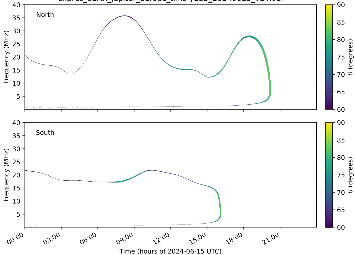
expres_earth_jupiter_europa_txka-y235_20240615_v14.cdf
