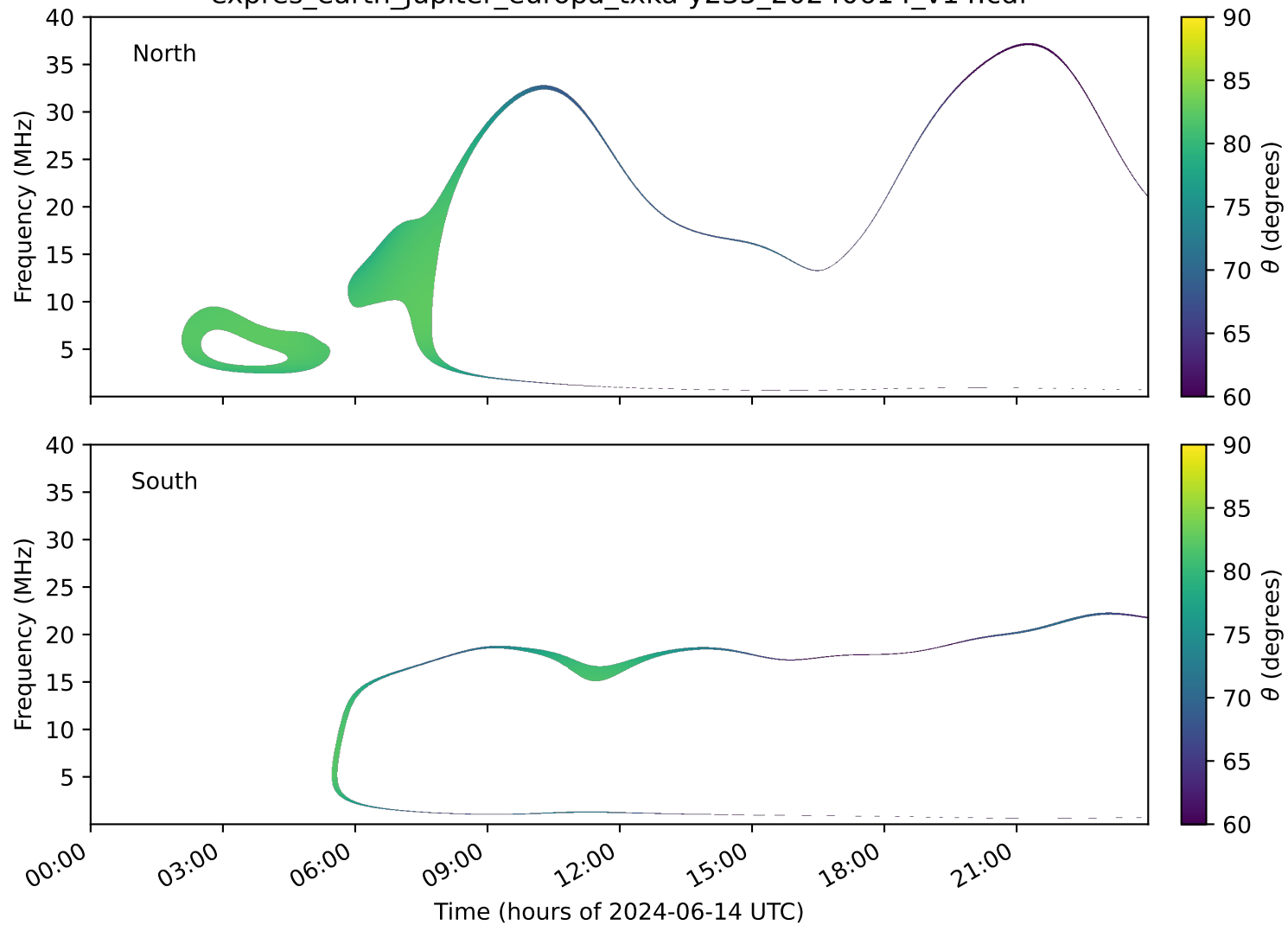
expres_earth_jupiter_europa_txka-y235_20240614_v14.cdf
