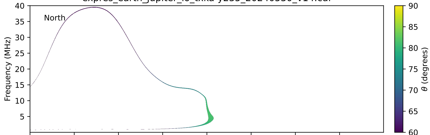
expres_earth_jupiter_io_txka-y235_20240530_v14.cdf
