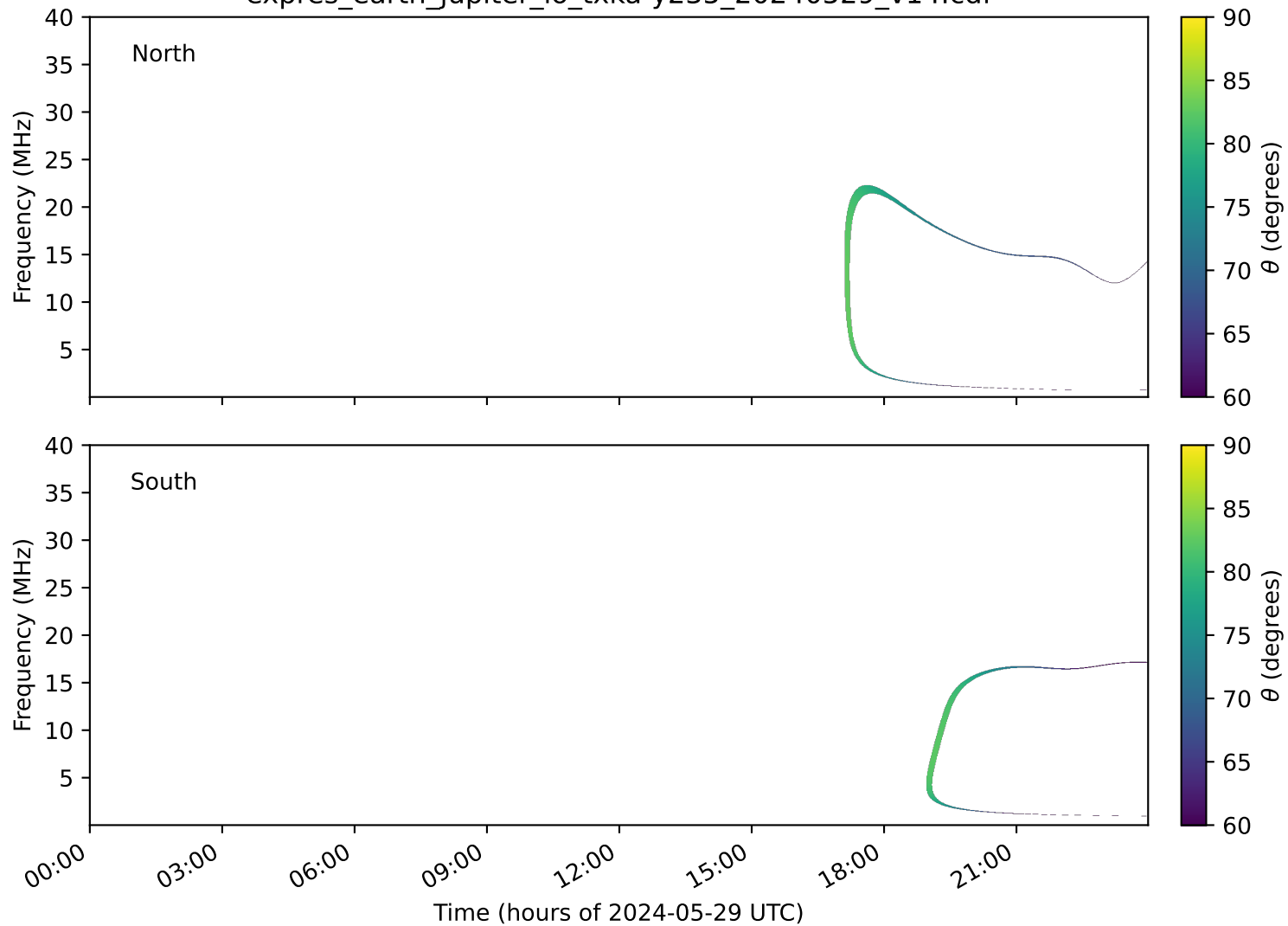
expres_earth_jupiter_io_txka-y235_20240529_v14.cdf
