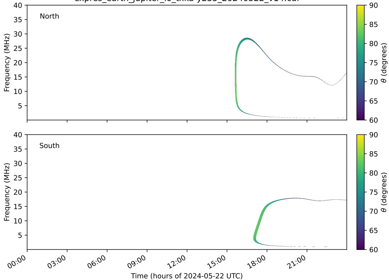
expres_earth_jupiter_io_txka-y235_20240522_v14.cdf
