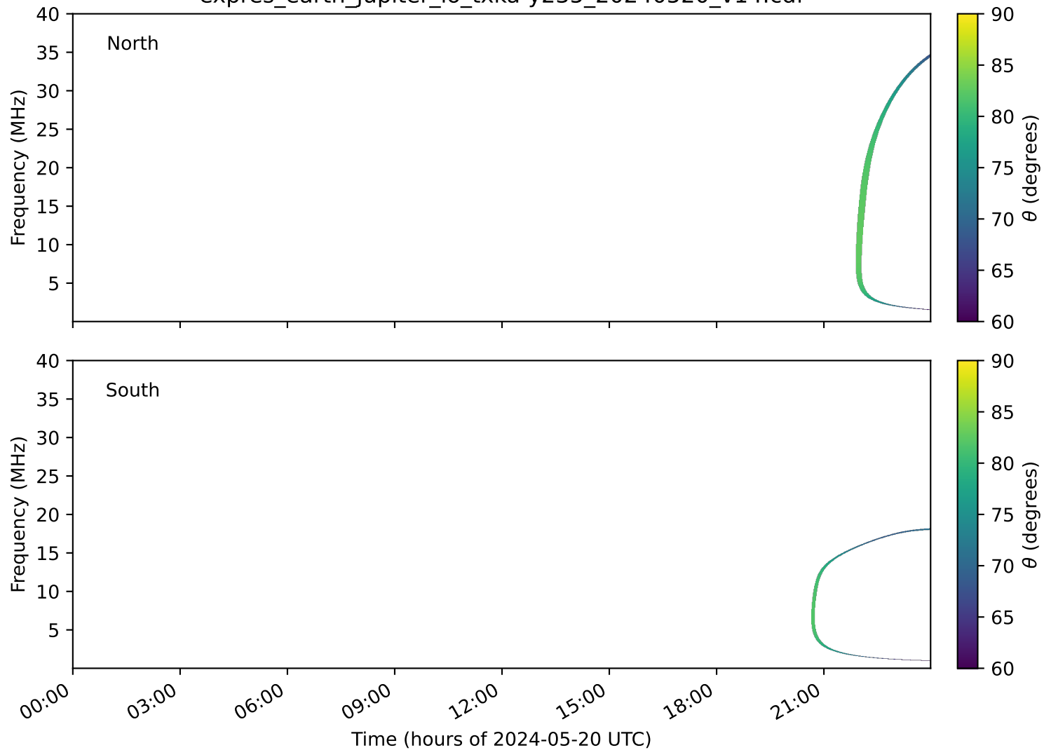
expres_earth_jupiter_io_txka-y235_20240520_v14.cdf
