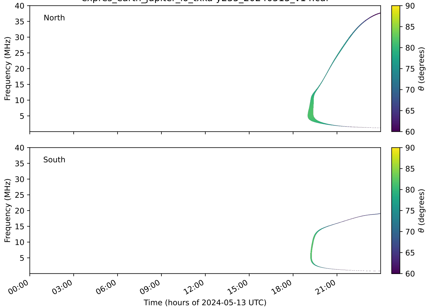
expres_earth_jupiter_io_txka-y235_20240513_v14.cdf
