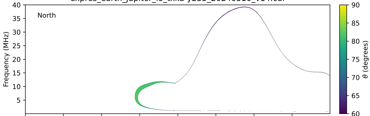
expres_earth_jupiter_io_txka-y235_20240510_v14.cdf
