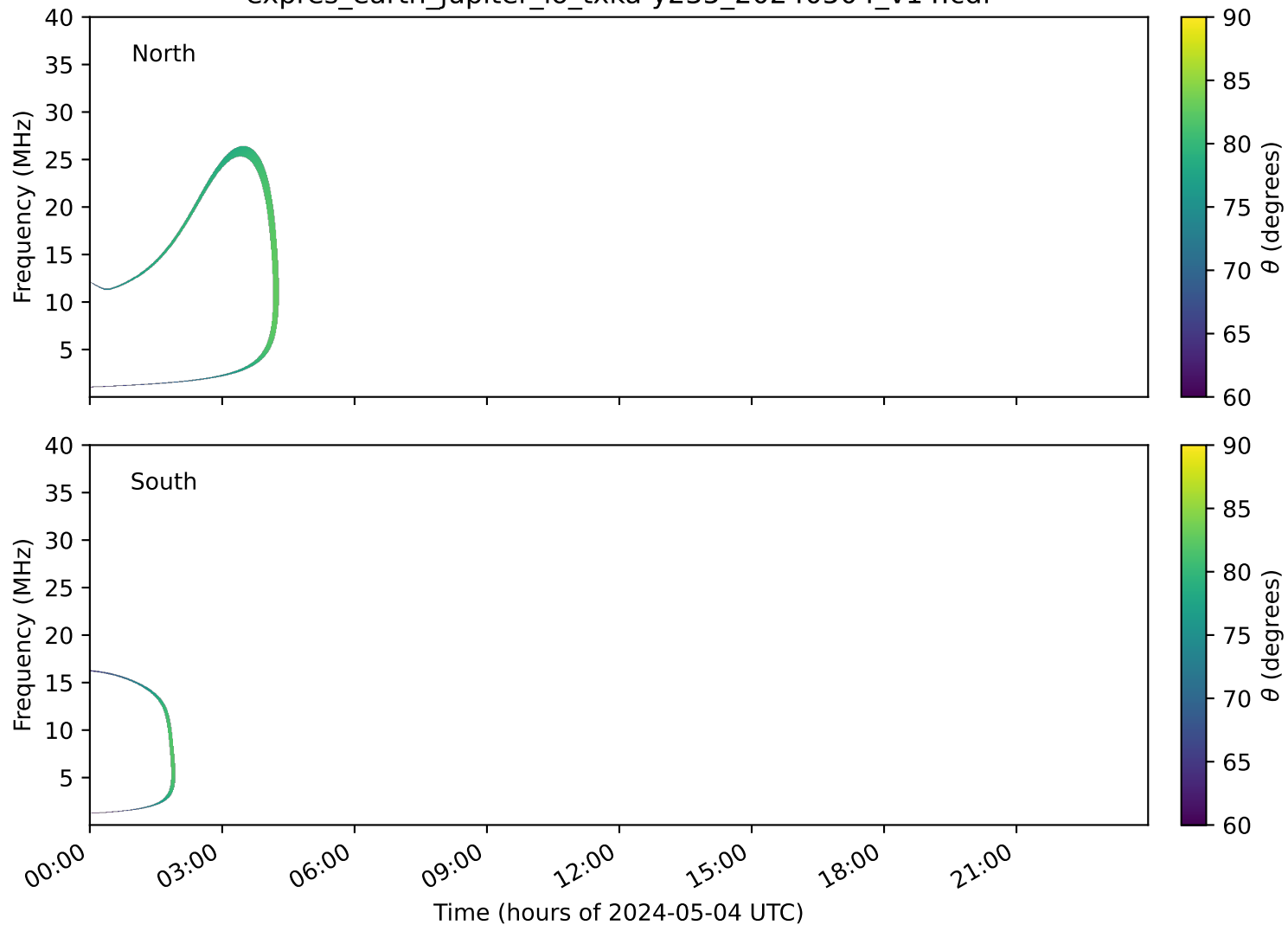
expres_earth_jupiter_io_txka-y235_20240504_v14.cdf
