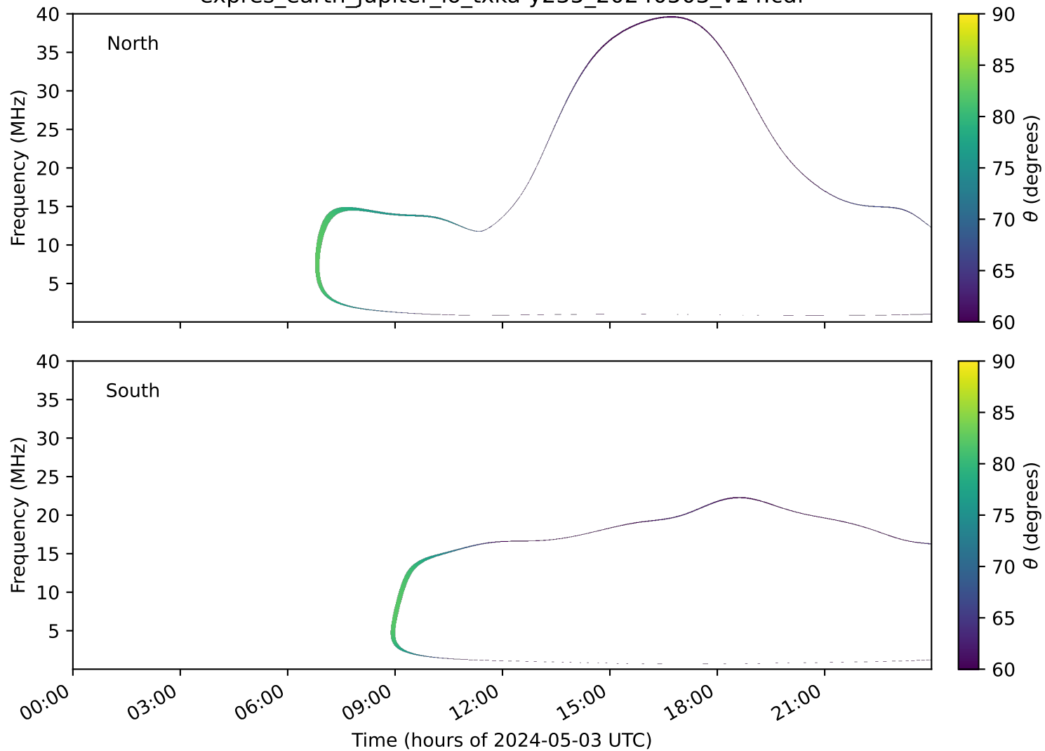
expres_earth_jupiter_io_txka-y235_20240503_v14.cdf
